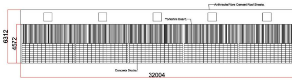
North Elevation.
