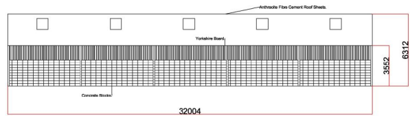
South Elevation.
